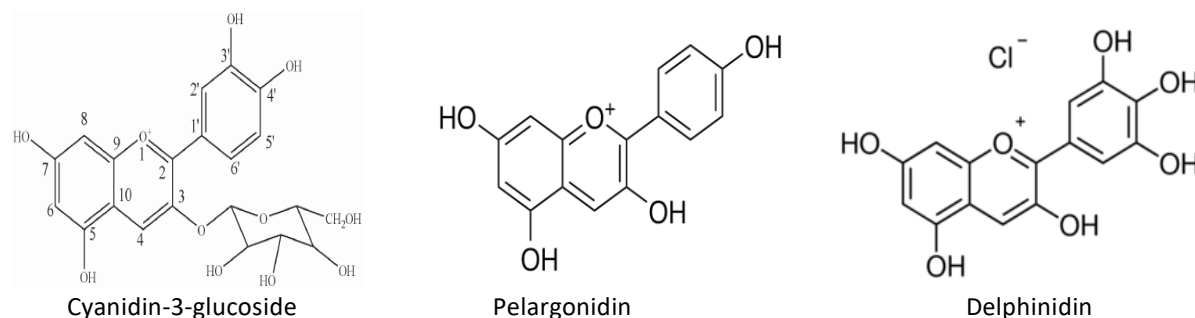
Figure 3. Structure of Standards
