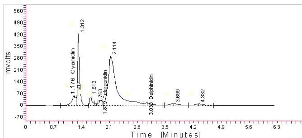
Figure 4. HPLC chromatogram of anthocyanins from red tamarind unripe fruit extract
