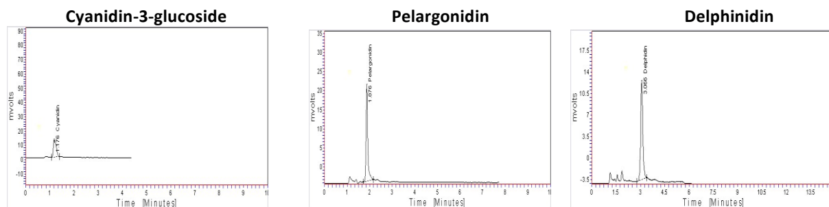
Figure 2. HPLC chromatogram of standards
