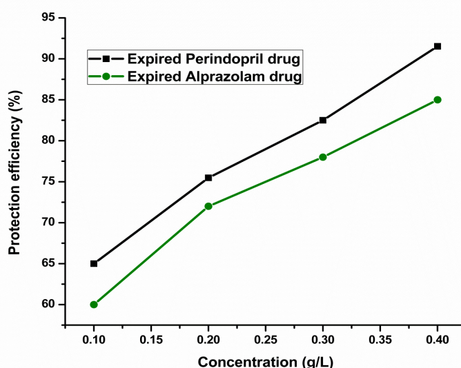
Figure 2: Protection efficiency of the corrosion inhibitors with four different amounts
