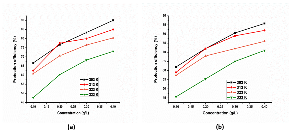
Figure 1: Protection efficiency of inhibitors (a) expired Perindopril drug, (b) expired Alprazolam drug
