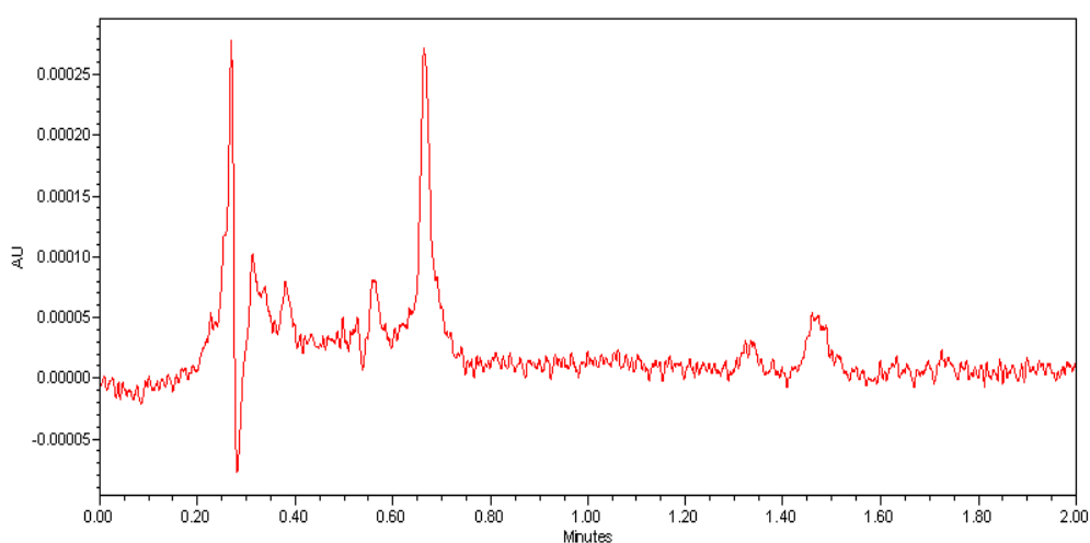
Fig: 3 Chromatogram of placebo
