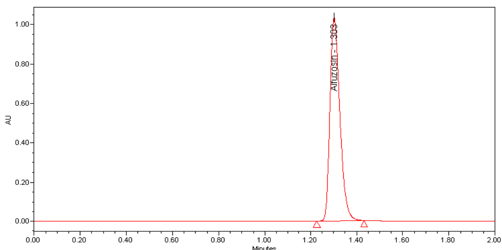
Fig: 4 Chromatogram of alfuzosin hydrochloride standard
