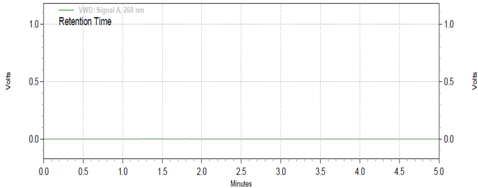
Blank Chromatogram
