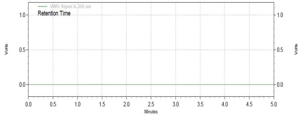
Placebo Chromatogram
