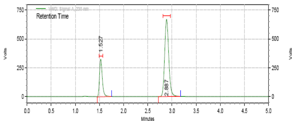
Accuracy chromatogram
