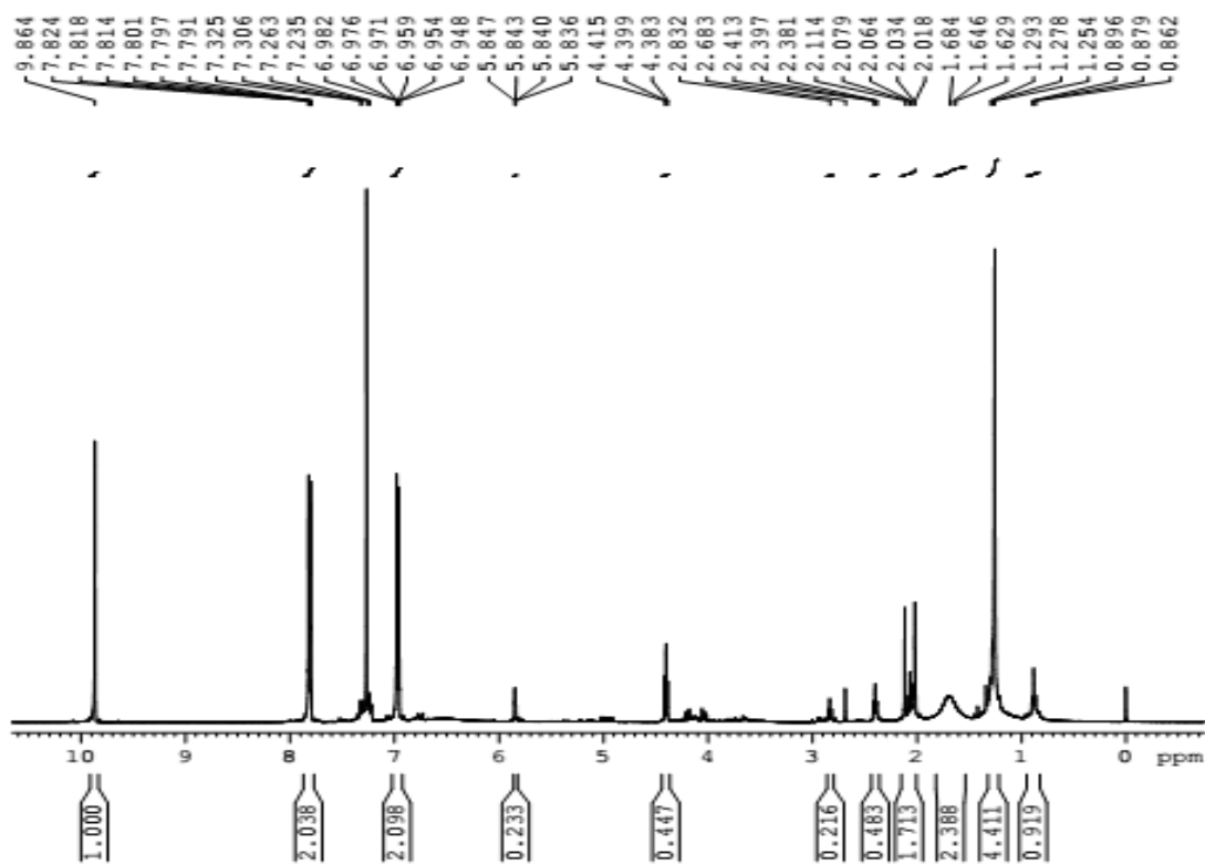
Fig. 2 1 H-NMR spectrum of the purified compound MJK-2
