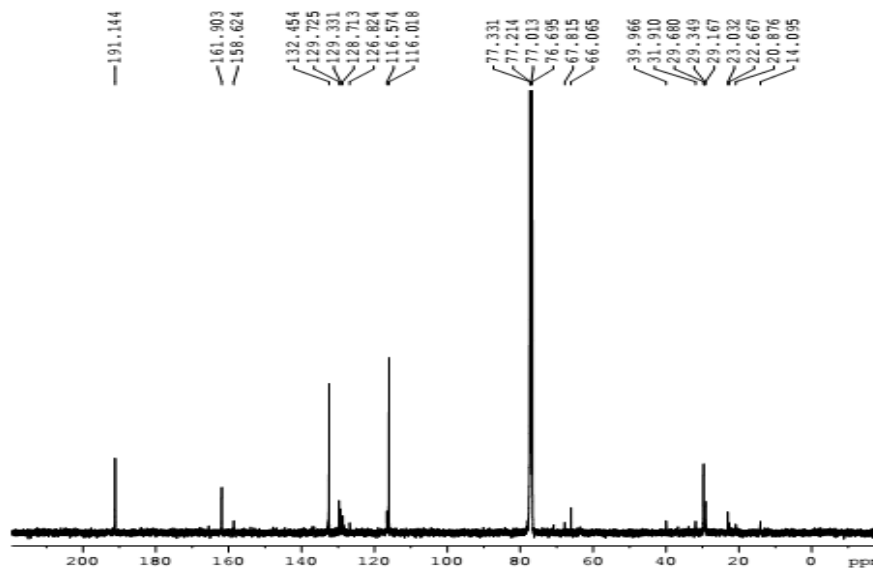
Fig. 4 Mass spectrum of the purified compound MJK-2
