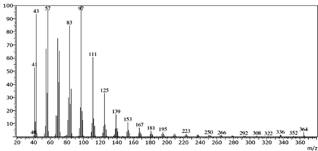
Fig. 5 Structure of the purified compound MJK-2
