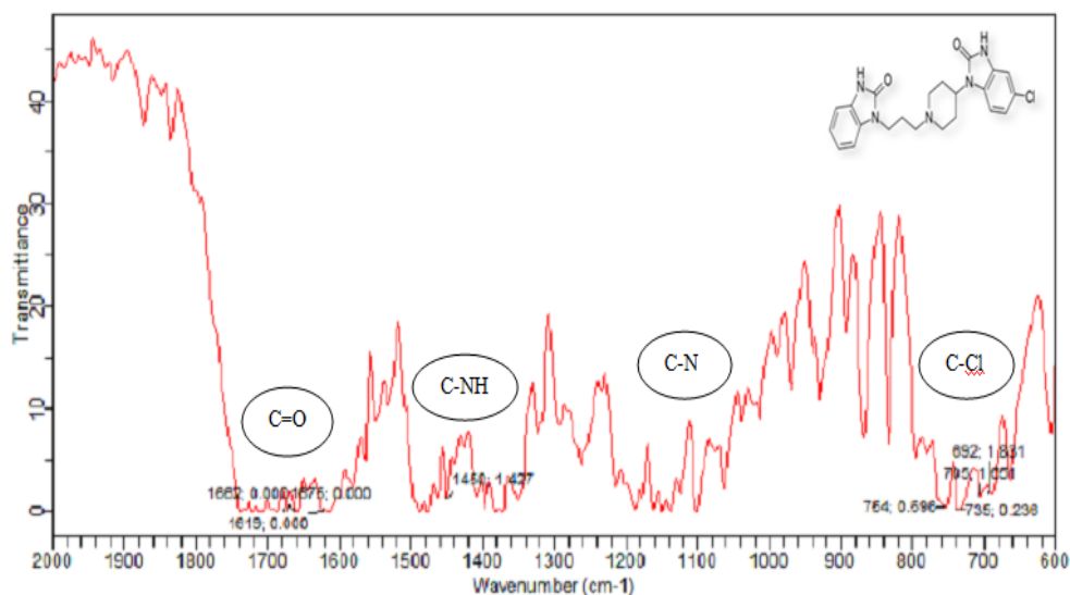
Figure 3: Spectra of Domperidone
