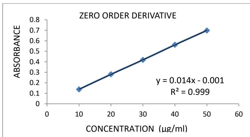
Fig. 4 Calibration curve of Propofol (Method A)
