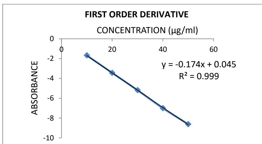
Fig. 5 Calibration curve of Propofol (Method B)
