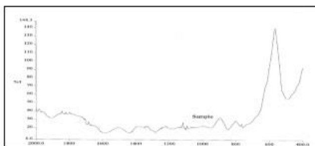
Fig No 2: FT- IR spectrum of Lansoprazole + Sodium Bicarbonate
