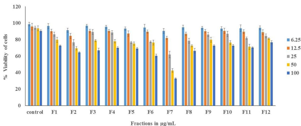
Fig 5: Cytotoxicity of fractions against Hep G2 cells by trypan blue exclusion method.
