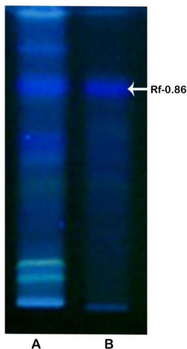
Fig 4: HPTLC chromatogram of ethyl acetate extract and bioactive fraction F7. A. ethyl acetate extract B. bioactive fraction 7. Showing Rf value of the purified metabolite.
