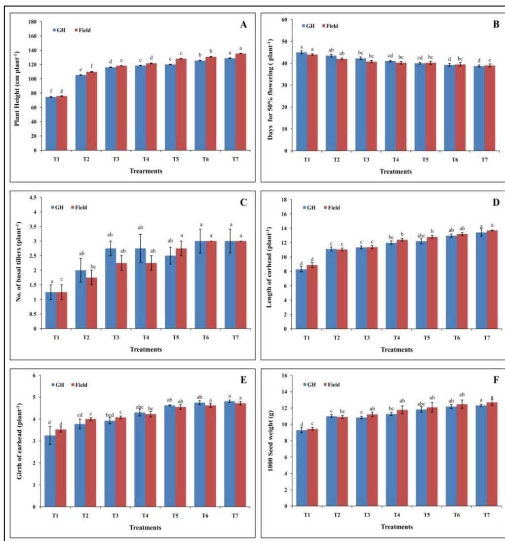
Figure 1: Effect of different elicitor treatments on plant growth parameters of pearl millet under greenhouse and field conditions. Each value is the mean for four replicates (n= 4) and bars sharing the same letters are not significantly different ( p \leq 0.05 ) according to Tukey's HSD. The vertical bar indicates the standard error.
