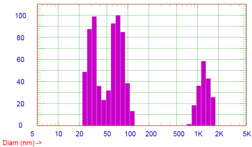
Figure 6: Particle size distribution of uncoated MNZ NPs
