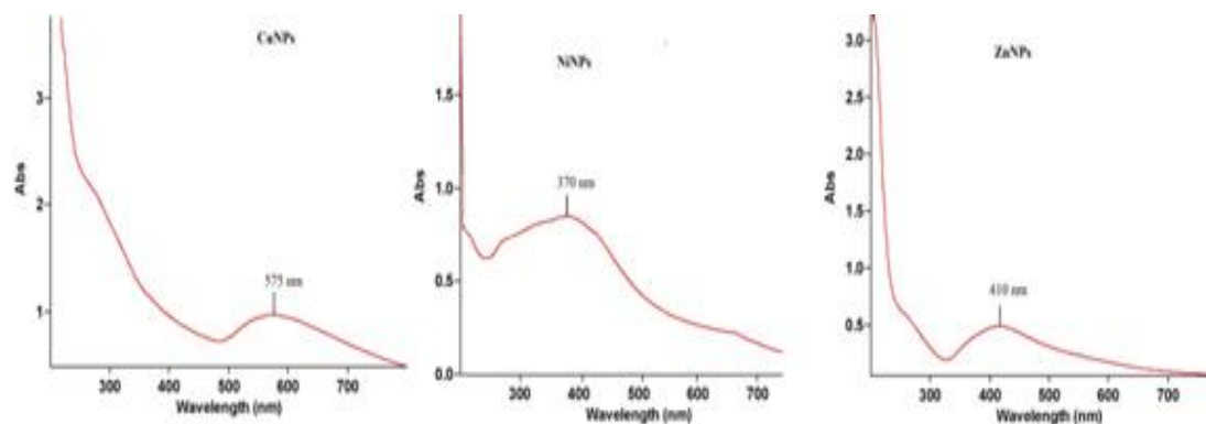
Figure 1: UV absorbance peaks of synthesized nanoparticles
