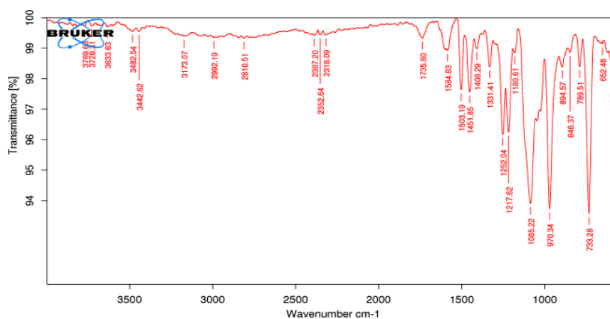
Figure 01: FT-IR spectrum of pure Carvedilol
