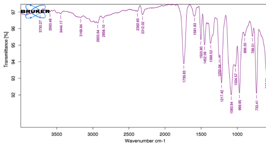
Figure 05: FT-IR spectrum of physical mixture of Carvedilol and Guar gum
