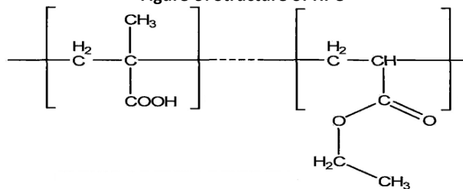
Figure 10: Structure of Kollicoat.
