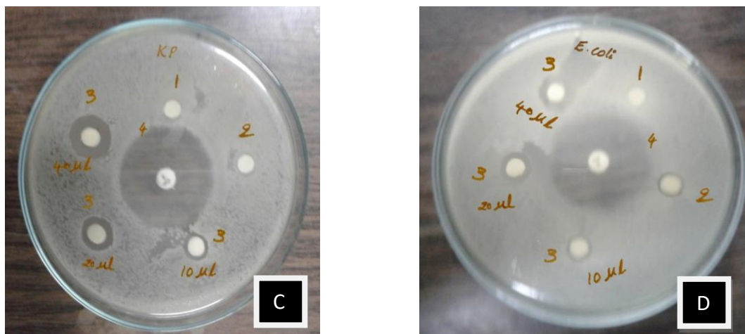
Fig.8 Antibacterial activity of Synthesized SNPs from whole plant extract of Gynura lycopercifolia . (A) Bacillus subtilis , (B) Staphylococcus aureus , (C) Klebsiella pneumoniae (D) Escherichia coli (1) Plant extract (2) \text{Ag}(\text{NO}_3)_2 (3) SNPs (4) Ciprofloxacin.
