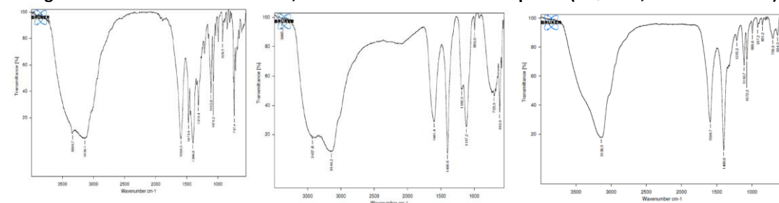
Fig 4: FTIR of CEFIXIME, CEFACTOR and CEFDINIR
