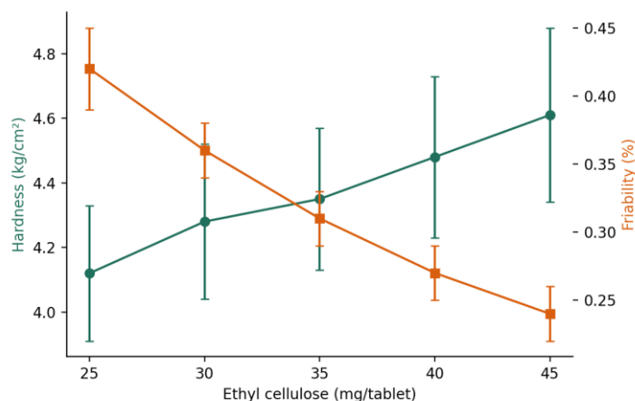
Figure 2. Effect of ethyl cellulose content on tablet hardness and friability (mean \pm SD).
