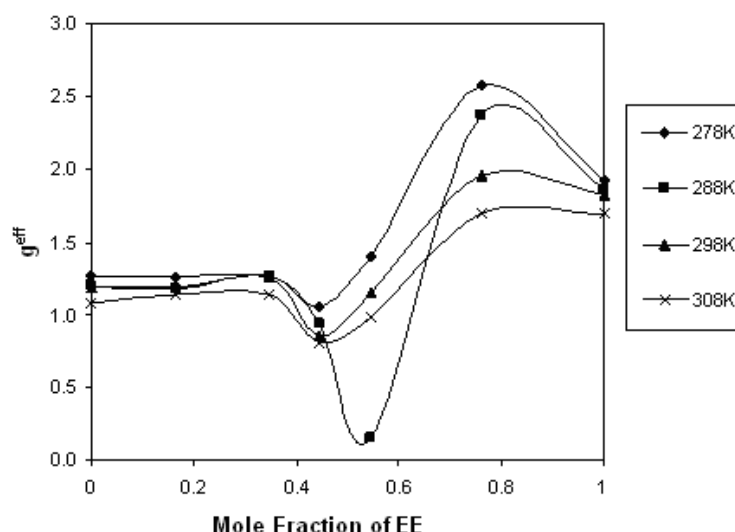
Graph 7: Variation of Kirkwood correlation factor g^{\text{eff}} as a function of mole fraction of Ethoxy Ethanol at different temperatures.
